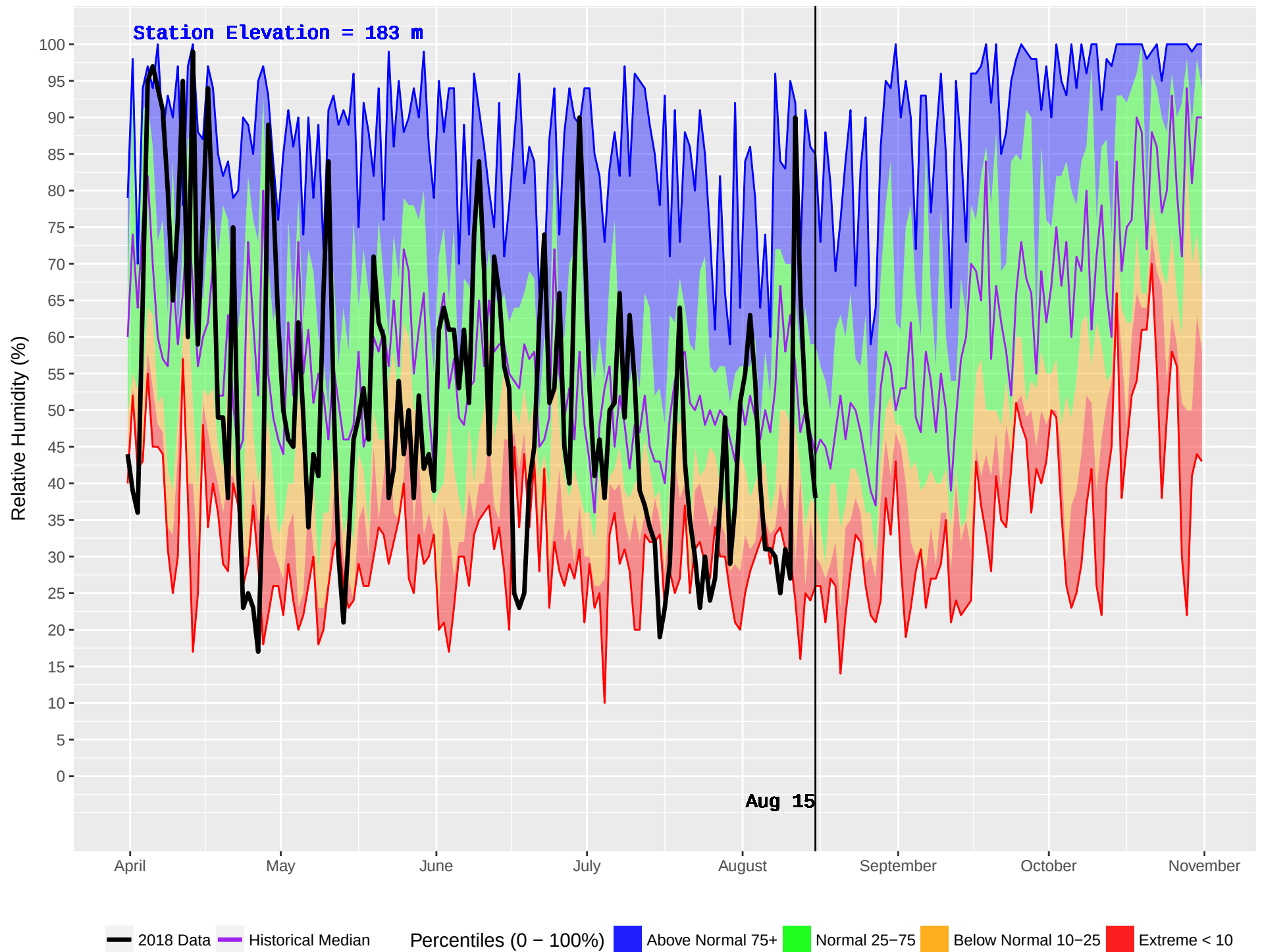
MESACHIE 2 (934) : Historical (2006–2016) and Current (2018) Daily Relative Humidity
