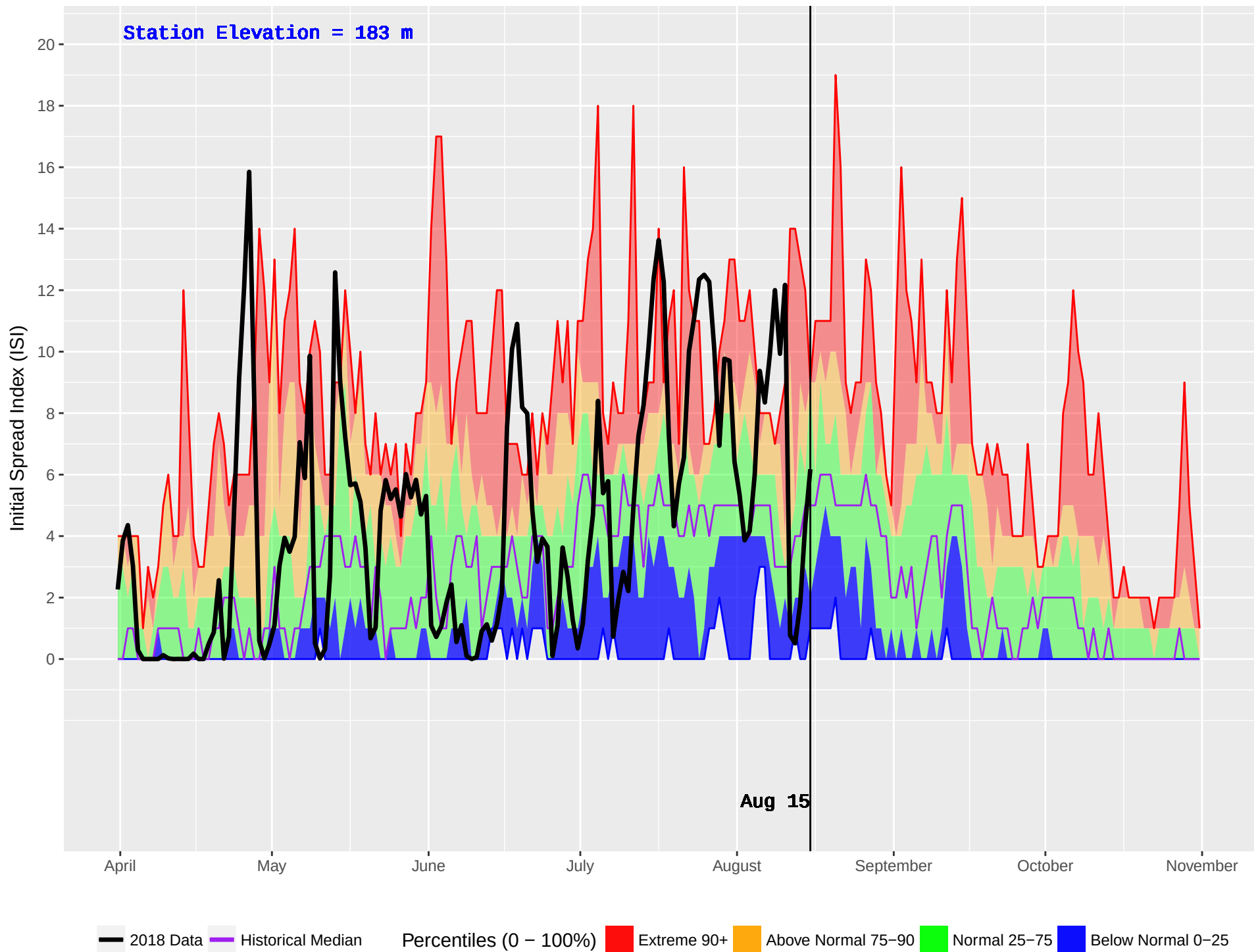
MESACHIE 2 (934) : Historical (2006–2016) and Current (2018) Daily Initial Spread Index (ISI)
