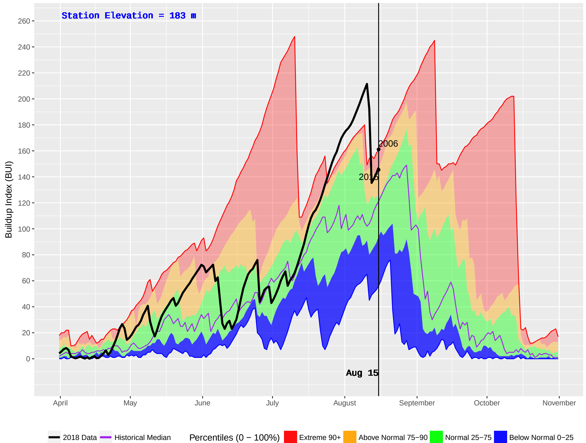
MESACHIE 2 (934) : Historical (2006–2016) and Current (2018) Daily Buildup Index (BUI)
