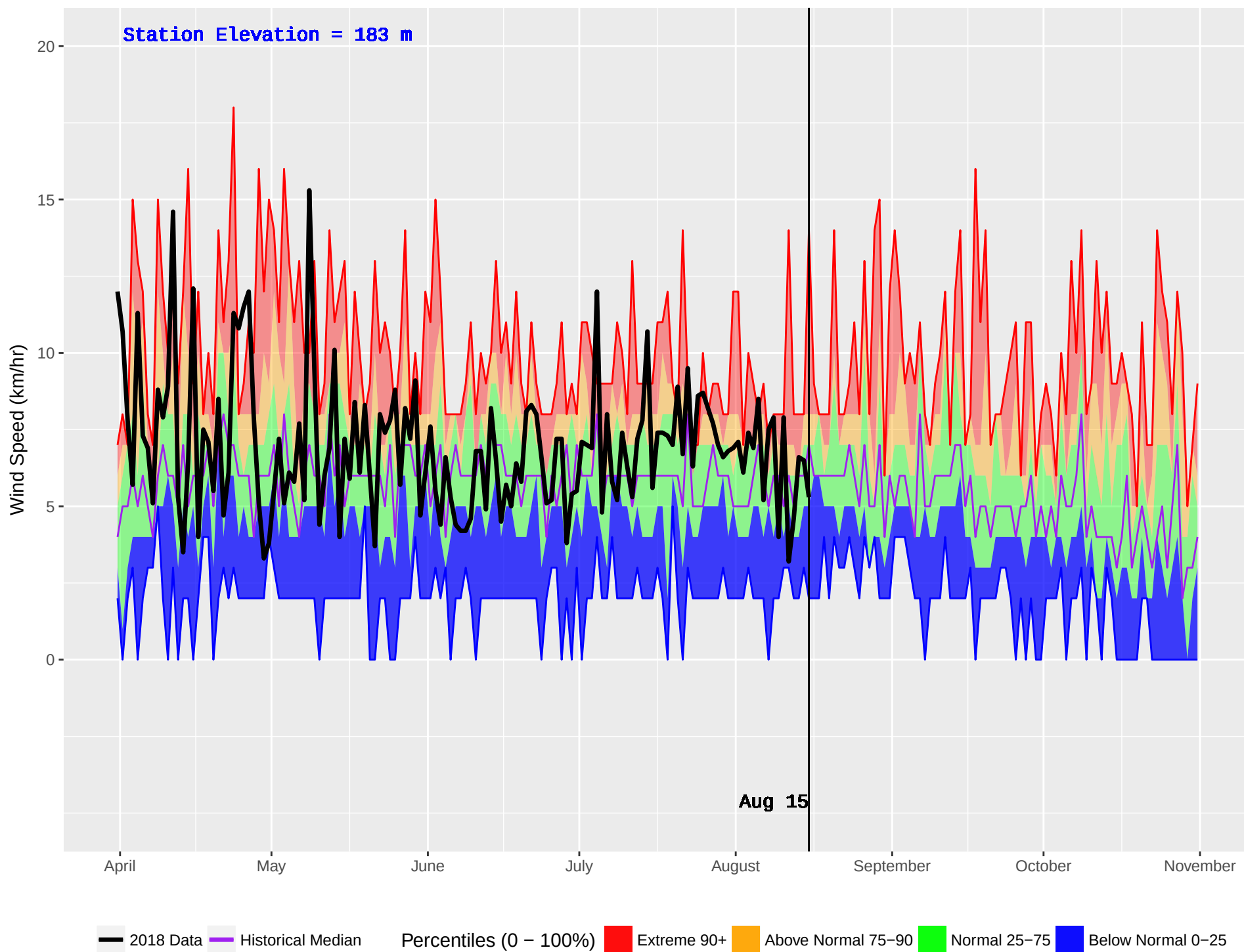
MESACHIE 2 (934) : Historical (2006–2016) and Current (2018) Daily Wind Speed
